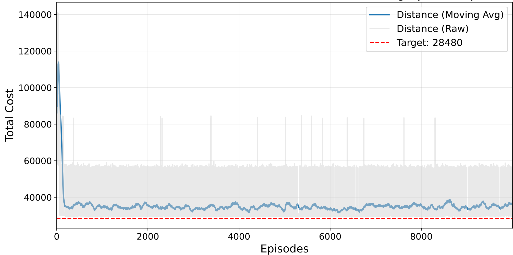
Final HYPERBAND TPE Masked AutoRL-SOP Training - p43.2.sop
